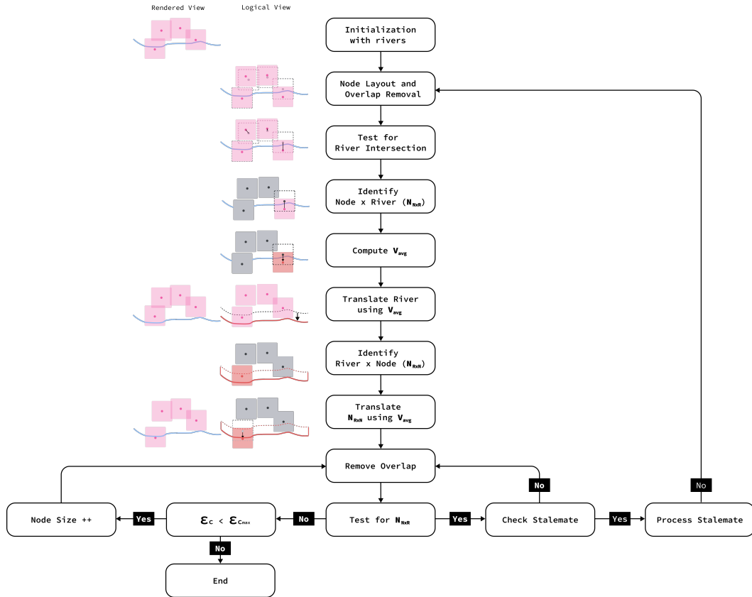
Figure 3. An overview of our hybrid layout algorithm incorporating rivers. See also Algorithm 3 in Section 4 for more detail. See Figure 5 for the logic of processing a stalemate. For illustration purposes, we show the rendered views alongside the logical views representing the actual computation, and use the same size for all squares for clarity.
