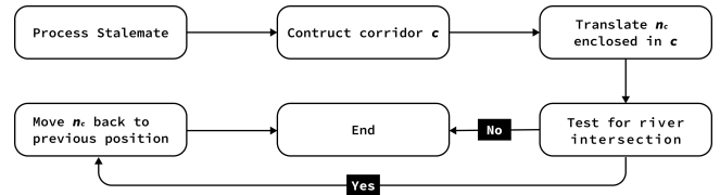
Figure 5. A flowchart illustration of stalemate processing. See Section 4.3, Figure 6, and Figure 7 for more detail. Refer to our video demonstration (from 1:27 to 1:46) † for details.
