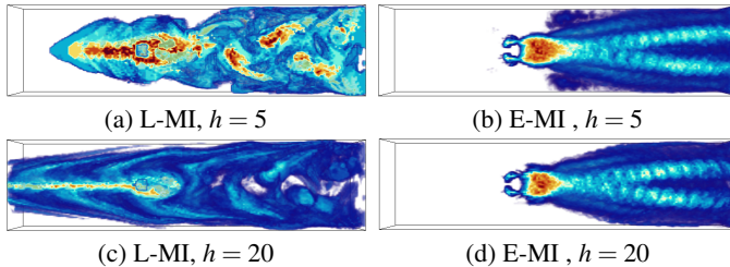
Fig. 11: Comparison of Lagrangian (L-) MI and Eulerian (E-) MI for the 3D cylinder data with different time windows h . (a) The left results are Lagrangian MI for acceleration and Q , and the right ones are Eulerian MI. We see that larger h makes both L.MI and E.MI smoother, but it does not change the structure of E.MI much.
