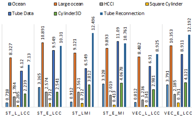
Fig. 13: Performance result for different metrics and different datasets.
