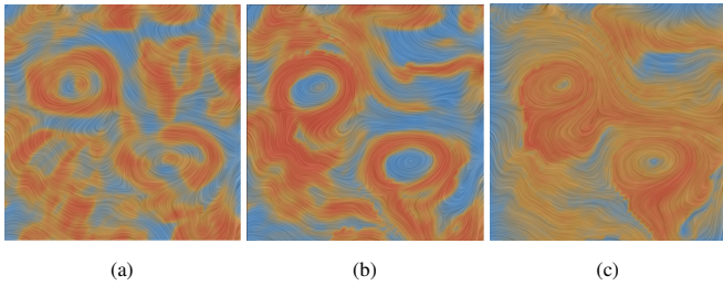
Fig. 2: Different correlation measurements of a region of the ocean simulation that contains eddies. (a) Spatial LCC, (b) Spatio-temporal (Lagrangian) LCC, and (c) mutual information (MI) (Lagrangian) between the Acceleration and Determinant of Jacobian matrix, respectively. For the first two results, the color shows the correlation characteristics, blue indicates negatively correlated and red positively correlated. For the MI result (c) blue indicates lower dependency and red indicates higher dependency.
