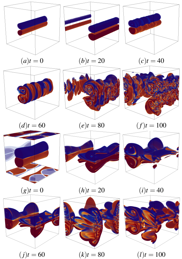
Fig. 12: The Spatial correlation for dye and vorticity for the elliptical instability simulation (a-f) and the Crow / reconnection simulation (g-l). In the top, we can see how the dye first tracks vorticity, until the non-linear elliptical instability kicks in and destroys the vortex, and the correlation is lost. In the bottom, we can see how the dye follows the vorticity much better even after the change in topology, and there is less mixture between red and blue regions. The spatial kernel size is 3.
