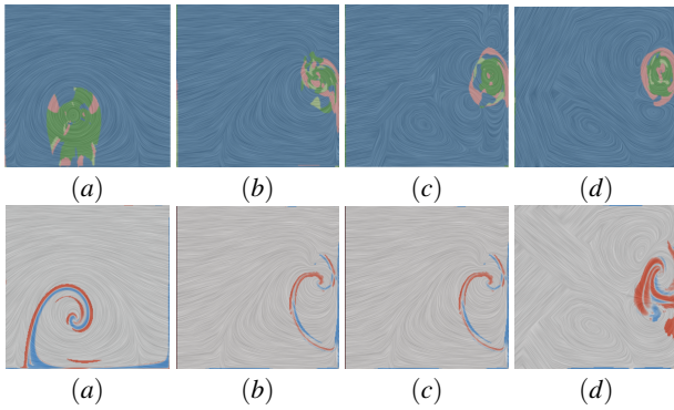
Fig. 9: The ranking based segmentation for the spatial correlation between pressure and other attributes over time. The green color indicates the regions where the correlation of pressure and vorticity is the highest, the pink color corresponds to the pair of pressure and kinetic energy, and blue for the pair of pressure and shearing. The second row of images show the result of ST_LCC for acceleration and kinetic energy. The results highlight regions similar to the FTLE ridges. The spatial kernel size is r = 3 and the temporal kernel size is h = 40 .
