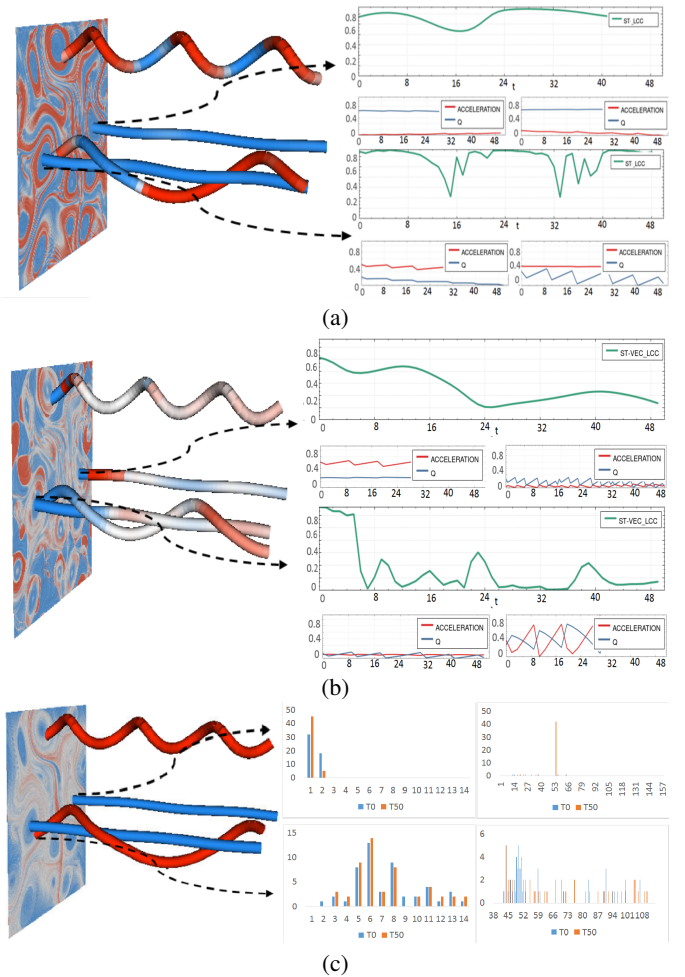
Fig. 4: Sampled pathlines colored based on the ST_LCC(a), ST_VEC_LCC(b) and MI(c) of acceleration and Q , respectively. Each top plot of (a) and (b) shows the ST_LCC/ST_VEC_LCC values along the respective pathlines indicated by the arrows. The two sub-plots beneath each large plot show the trends of the two given attributes within a kernel. For the MI result (c), the left two histograms show the distributions of the attribute values of Q within kernels on two pathlines (indicated by the arrows), while the right two show the distributions of the values of acceleration within the same kernels. Each histogram shows two distributions of the values of the respective attribute within two different kernels sampled at t=0 (blue) and t=50 (orange) on the corresponding pathline, respectively. Since we used equal-width bins, the number of bins are different for different attributes.
