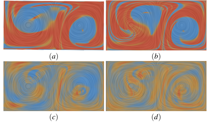
Fig. 15: The effect of different temporal kernel sizes for ST_LCC (a-b) and MI (c-d) computation. The temporal kernel sizes are 50 (left column) and 100 (right column), respectively, considering \tau = 0.05 .
