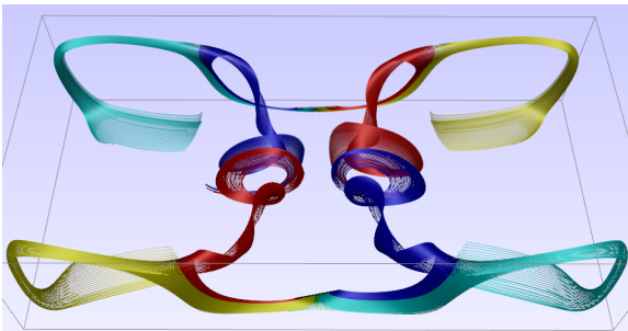
Fig. 5. Our similarity measures and clustering algorithm segment the streamlines on this rake into distinct, intuitive clusters. Two rakes were used to generate two sets of streamlines on a simulation of Bénard convection in this image. Color indicates cluster membership. Note colors are re-used for each rake (i.e. the two red clusters are distinct clusters).
