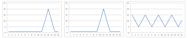
Fig. 6. Test streamlines for the hierarchical algorithm. Left: A streamline with a high peak towards the end. Middle: A shifted version of the top streamline. Right: A dissimilar streamline.
