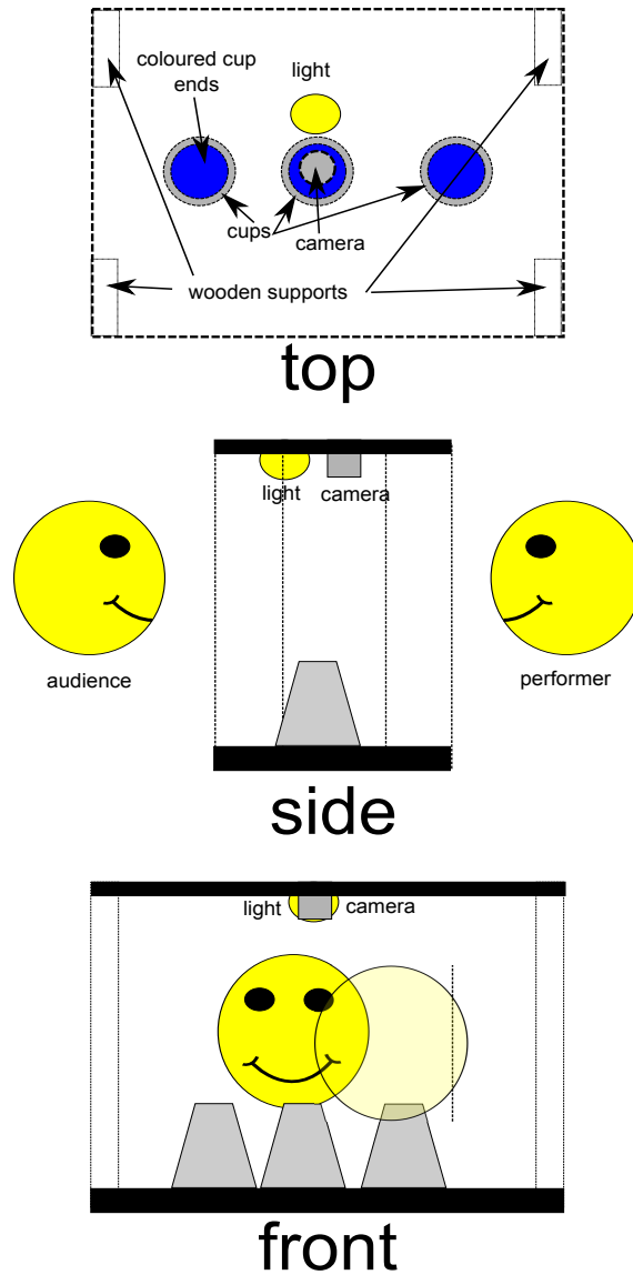
Figure 5.4: Schematic of the Cup Table
