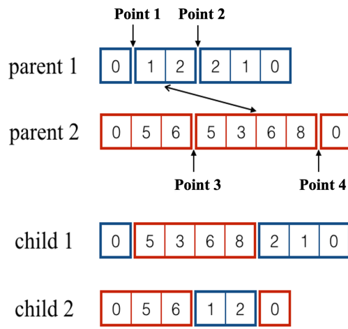
Figure 4 Examples of crossover operators in the GA
