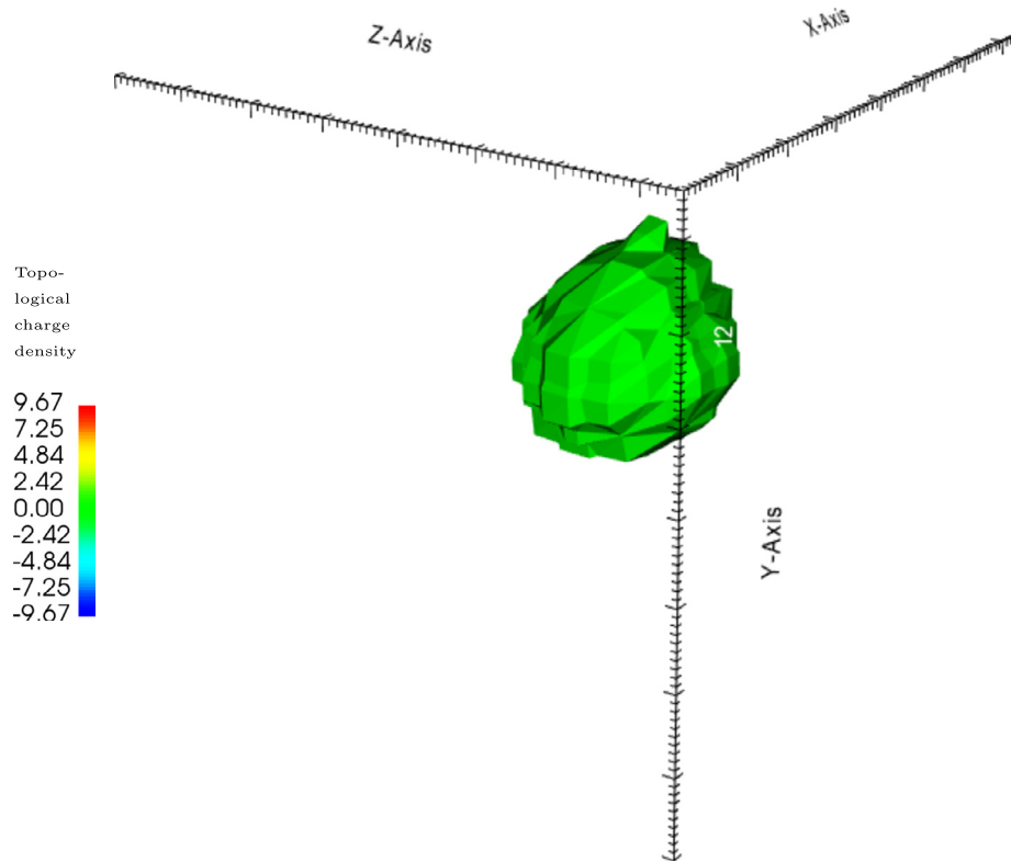
Fig. 20. The slab structure of the instanton recovered from the JCN of t = (1, 2, 3, 4, 5, 6, 7, 8) .
