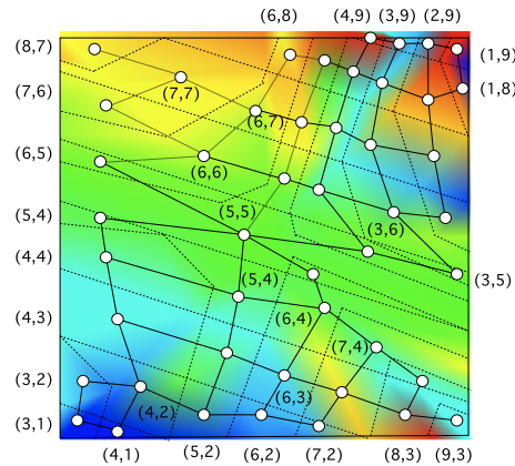
Fig. 2. The JCN capturing the bivariate topology of the two simple functions shown in Fig. 1. The bivariate field is decomposed by overlaying the quantisation intervals of the two input fields (dotted line). A vertex is placed at the barycentre of each region, or joint contour slab, and edges mark adjacency. Image taken from Duke et al. [5].
