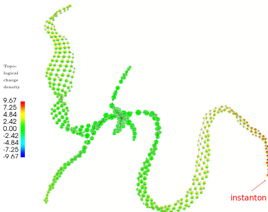
Fig. 10. An instanton can be located in the t = (5, 6) JCN as the branch with red & yellow glyphs. The bottom half of the glyphs indicate that the topological charge density quickly drops off from a global peak at t = 5 .
