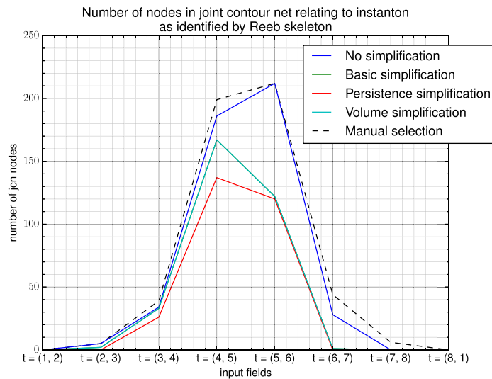
Fig. 17. Number of nodes in the JCN representing the instanton under simplification.
