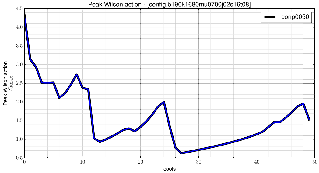
Fig. 6. Peak Wilson action S_{PEAK} .
