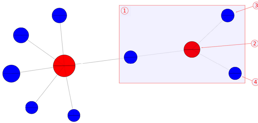
Fig. 14. Reeb skeleton for t = (5, 6) , simplified using volume persistence measures. The instanton (1) is captured as a branch in the simplified Reeb skeleton. At vertex (2) the instanton splits into two; the outer part (3) and inner core (4).
