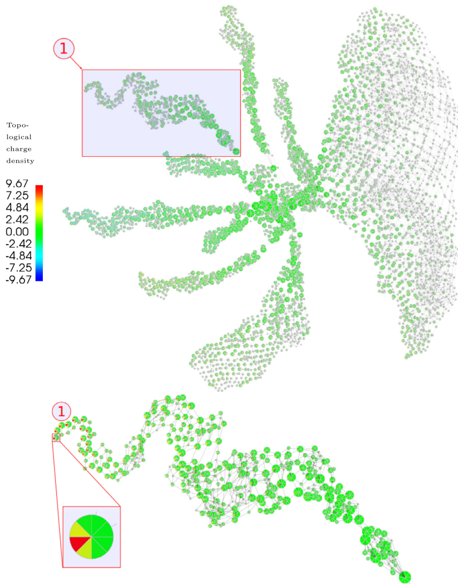
Fig. 19. Top: The JCN for t = (1, 2, 3, 4, 5, 6, 7, 8) . captures the instanton as branch (1). Bottom: Examining the branch in greater detail shows that the peak in topological charge density is captured in only a few vertices at the end of the branch. The peak in the topological charge density is captured by the multivariate glyph at t = 5 . It is also possible to observe elevated levels in the topological charge density in neighbouring time slices.
