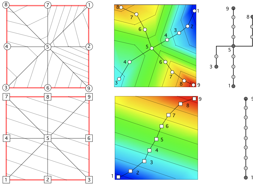
Fig. 1. Two simple scalar functions defined on a simplicial grid (left) where the dotted lines represent the quantisation intervals. The quantised contour tree for each function (right) is shown mapped to scalar field in the centre. Image taken from Duke et al. [5].
