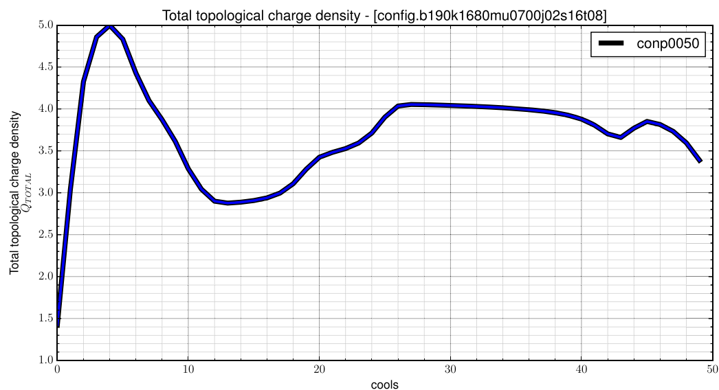
Fig. 5. Total topological charge Q_{TOT} .
