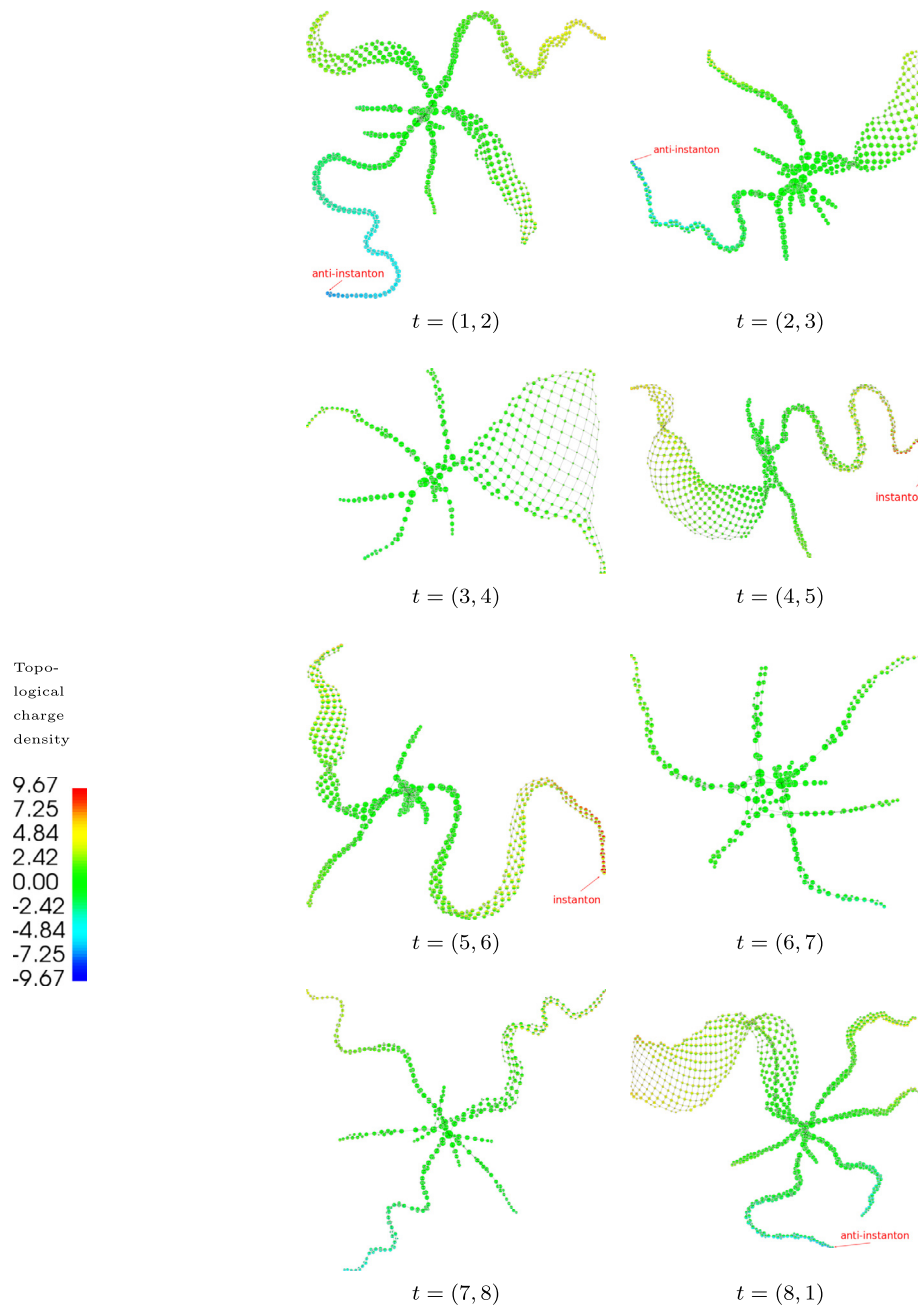
Fig. 8. Using the JCN to locate the most prominent (anti-)instantons (by magnitude) across the time axis. Less prominent (anti-)instantons also appear in the data but are not labelled.
