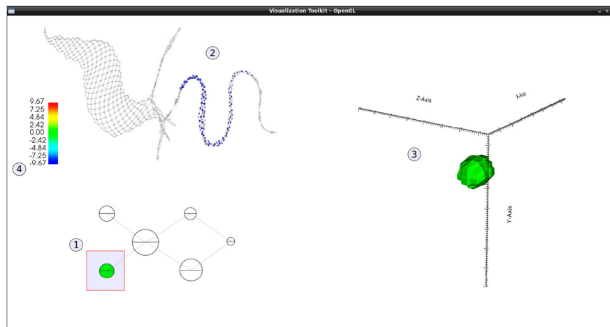
Fig. 4. The user interface allows the user to select nodes in the Reeb skeleton (1) or JCN (2) using rubber band selection. Green glyphs in the Reeb skeleton correspond directly to the blue glyphs in the JCN view. Selected vertices are displayed as quantised contours (3) using a colour transfer function (4) determined by the bivariate input fields.
