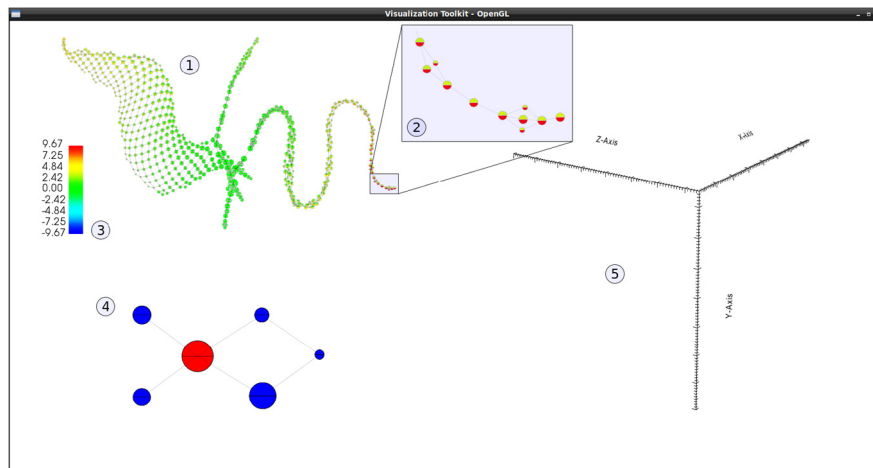
Fig. 3. The user interface used to explore temporal lattice QCD data as captured by the JCN. The JCN captures the topology as a graph structure (1) – displayed here in a spring layout. Each JCN glyph (2) represents a slab (or quantised contour) using scale to provide feedback on the overall size of the slab. Glyphs are coloured by isovalue (3), where the top half of each glyph represents the first input field and the bottom the second input. Also visible is the Reeb skeleton (4) which captures the JCN in a simplified form; red glyphs represent major changes in topological connectivity and blue glyphs represent relatively stable regions of topological structure. Slabs are only rendered (5) to reflect any selections made by the user; in this view nothing has been selected. (For interpretation of the colours in the figure(s), the reader is referred to the web version of this article.)
